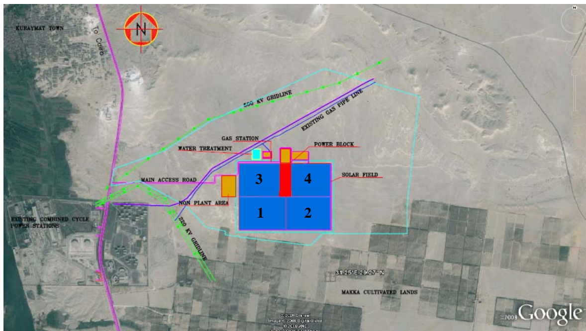
Figure 4-1 Plant Overview
